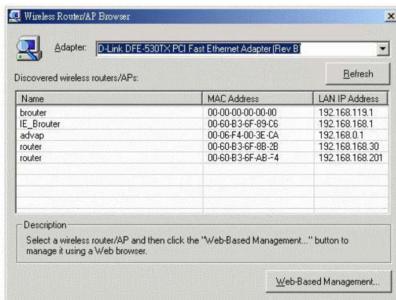
Rys. 32. Wireless Router/AP Browser.
